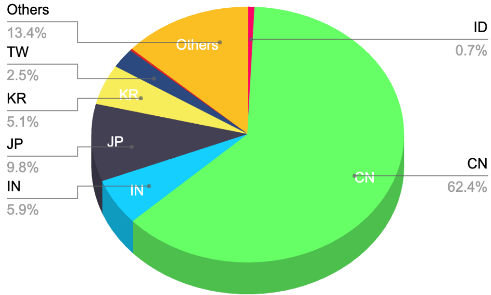
IPv6 delegations
