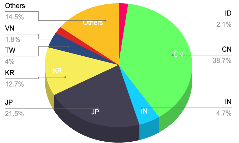
IPv4 delegations
